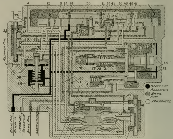
FIG. 1 FULL RELEASE POSITION—BRAKE PIPE RESERVOIR CHARGING TRIPLE VALVE IN QUICK RELEASE
